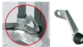
VSG1000A18 Bead pushing roller
